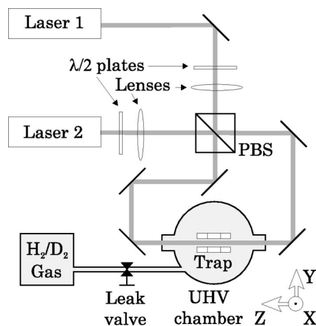
FIG. 1. Sketch of the experimental setup. The \lambda/2 plates and the polarization beam splitter (PBS) are used to balance the radiation pressure forces.
