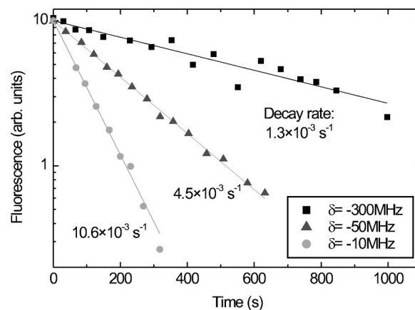
FIG. 3. Data series representing the total fluorescence from the ^{24}\text{Mg}^+ ions as a function of time during a \text{D}_2 gas load for various laser detunings \delta from the 3s^2S_{1/2} - 3p^2P_{3/2} transition. The lines represent fits to exponential decays with a constant background.
