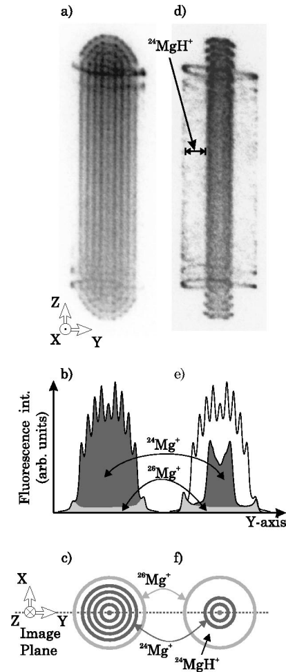
FIG. 2. (a) CCD pictures of fluorescence from ^{24}\text{Mg}^+ and the ^{26}\text{Mg}^+ ions in an ion crystal before introduction of \text{H}_2 gas. (b) Fluorescence distributions obtained by integration of the fluorescence signal from (a) along the z axis. (c) A sketch showing the ion crystal shell structure in the x - y plane, with a core of ^{24}\text{Mg}^+ ions and an outermost shell of ^{26}\text{Mg}^+ ions. In (b), the contributions from the two isotopes to the fluorescence signal are indicated by the two gray scales. (d), (e), and (f) correspond to (a), (b), and (c), respectively, but after \text{H}_2 gas loading (see the text for more details). The molecular ^{24}\text{MgH}^+ ions fill the region between the fluorescing core ( ^{24}\text{Mg}^+ ) and the outermost shell ( ^{26}\text{Mg}^+ ). In (e) the integrated fluorescence distribution from (b) is shown for comparison.
